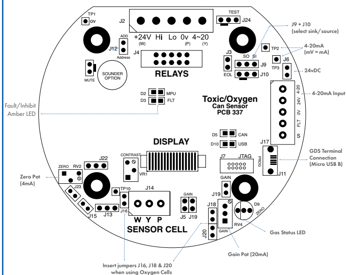
Fig. 1 Transmitter
